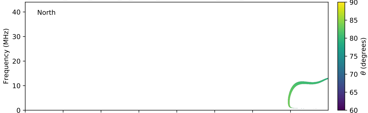
expres_earth_jupiter_io_jrm09_lossc-wid1deg_3kev_20050709_v01.cdf
