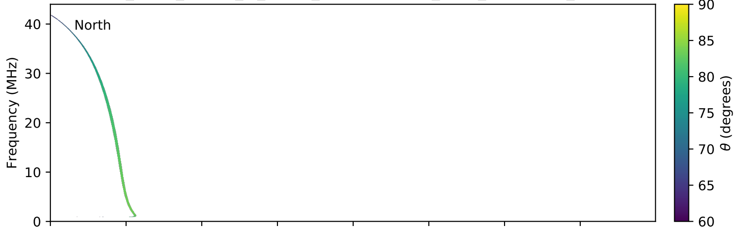
expres_earth_jupiter_io_jrm09_lossc-wid1deg_3kev_20050707_v01.cdf
