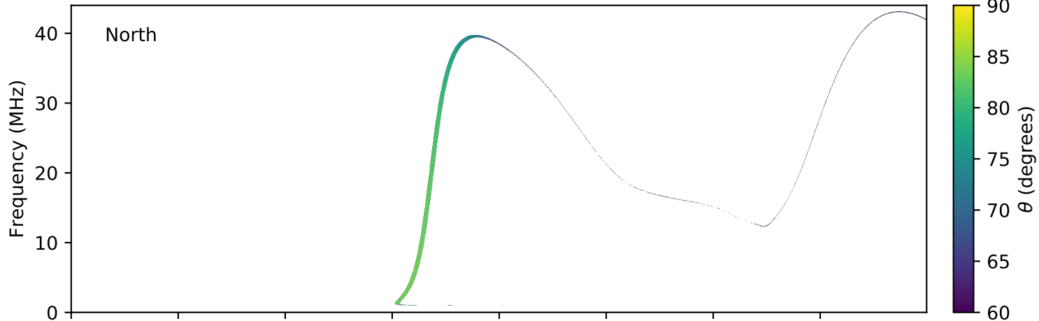
expres_earth_jupiter_io_jrm09_lossc-wid1deg_3kev_20050706_v01.cdf
