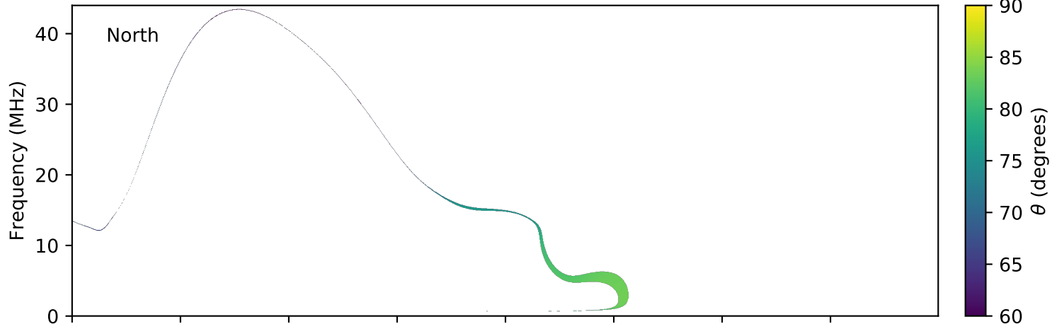
expres_earth_jupiter_io_jrm09_lossc-wid1deg_3kev_20050703_v01.cdf
