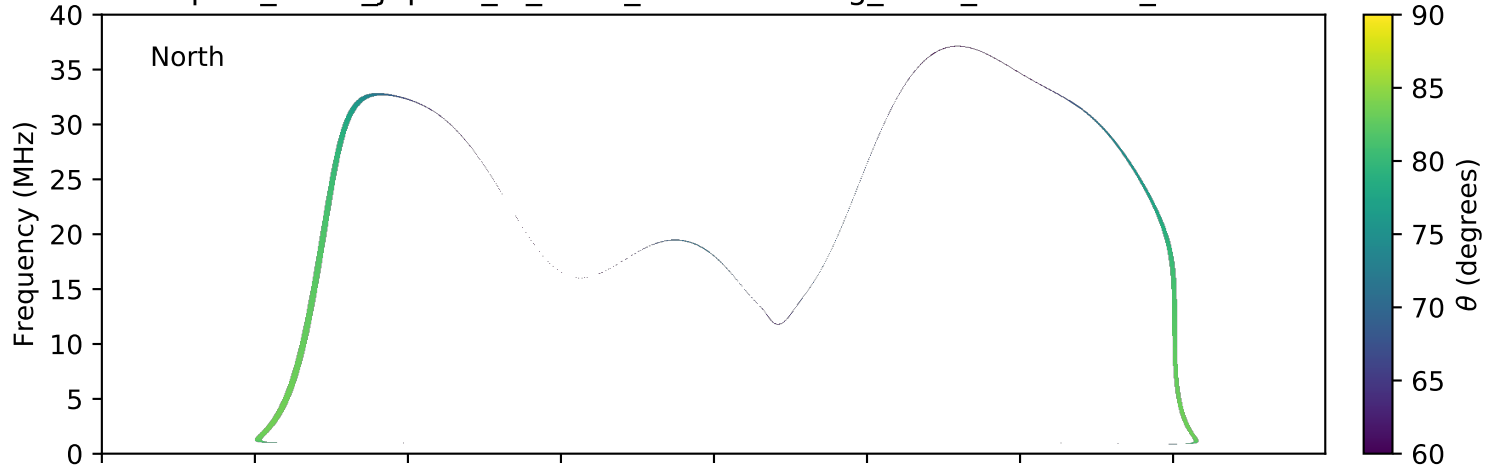
expres_earth_jupiter_io_isaac_lossc-wid1deg_3kev_20050731_v01.cdf
