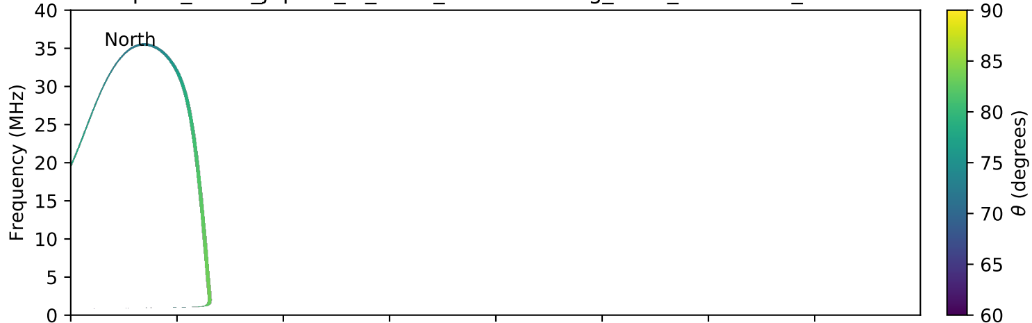
expres_earth_jupiter_io_isaac_lossc-wid1deg_3kev_20050730_v01.cdf
