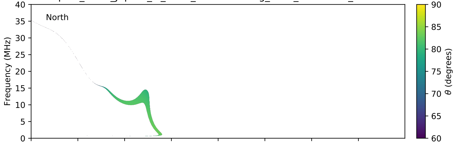
expres_earth_jupiter_io_isaac_lossc-wid1deg_3kev_20050728_v01.cdf
