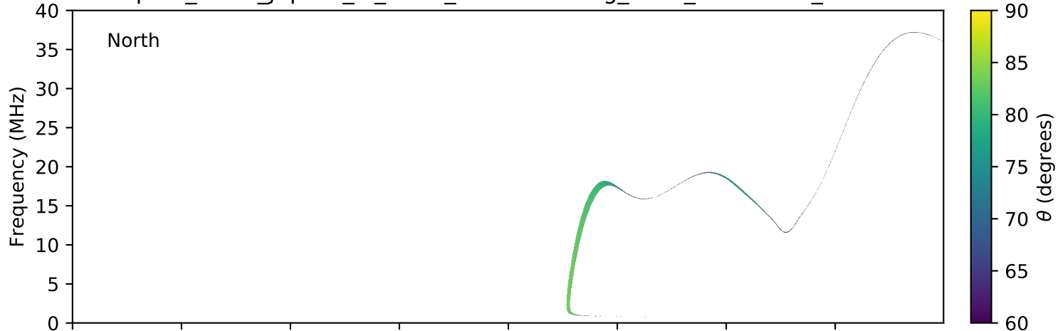
expres_earth_jupiter_io_isaac_lossc-wid1deg_3kev_20050727_v01.cdf
