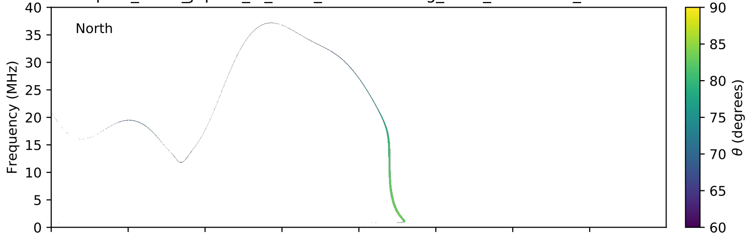
expres_earth_jupiter_io_isaac_lossc-wid1deg_3kev_20050726_v01.cdf
