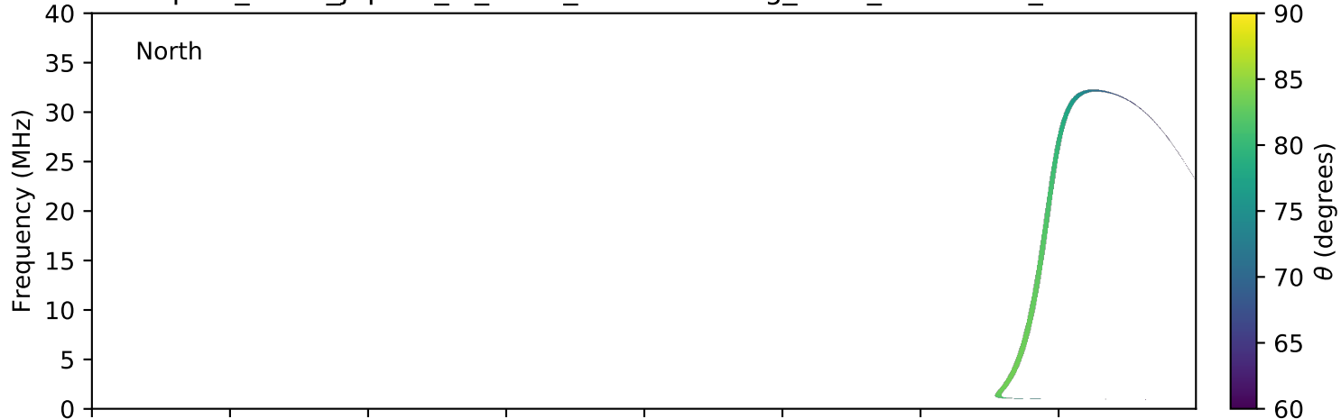
expres_earth_jupiter_io_isaac_lossc-wid1deg_3kev_20050725_v01.cdf
