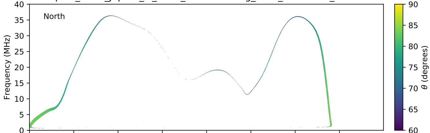
expres_earth_jupiter_io_isaac_lossc-wid1deg_3kev_20050724_v01.cdf
