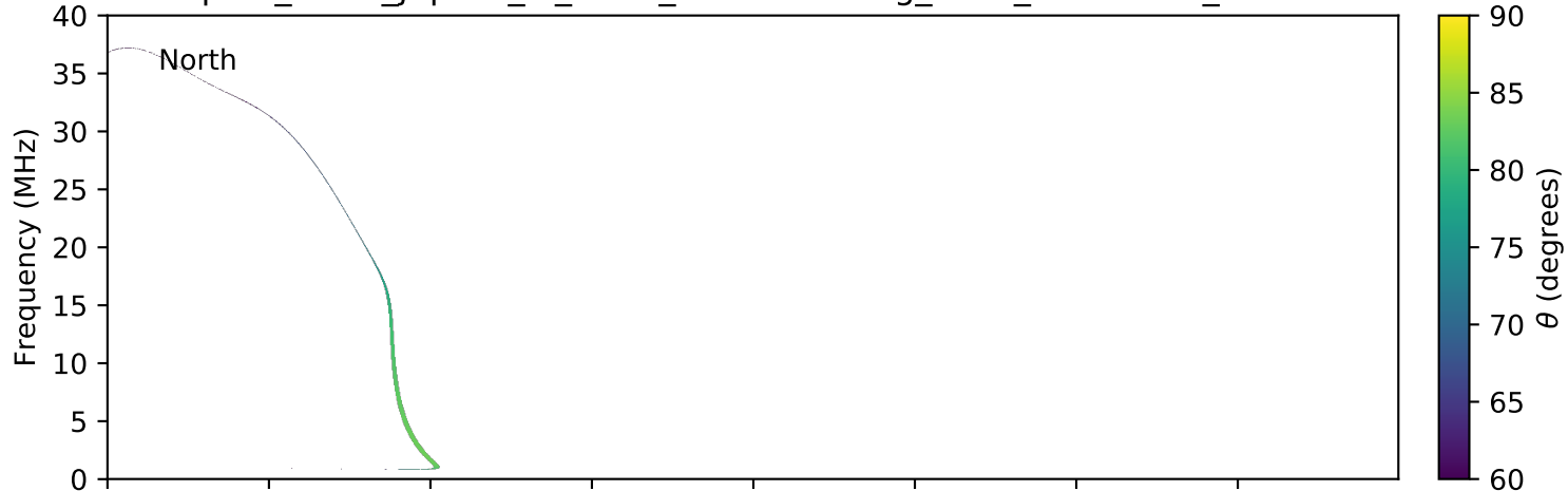
expres_earth_jupiter_io_isaac_lossc-wid1deg_3kev_20050721_v01.cdf
