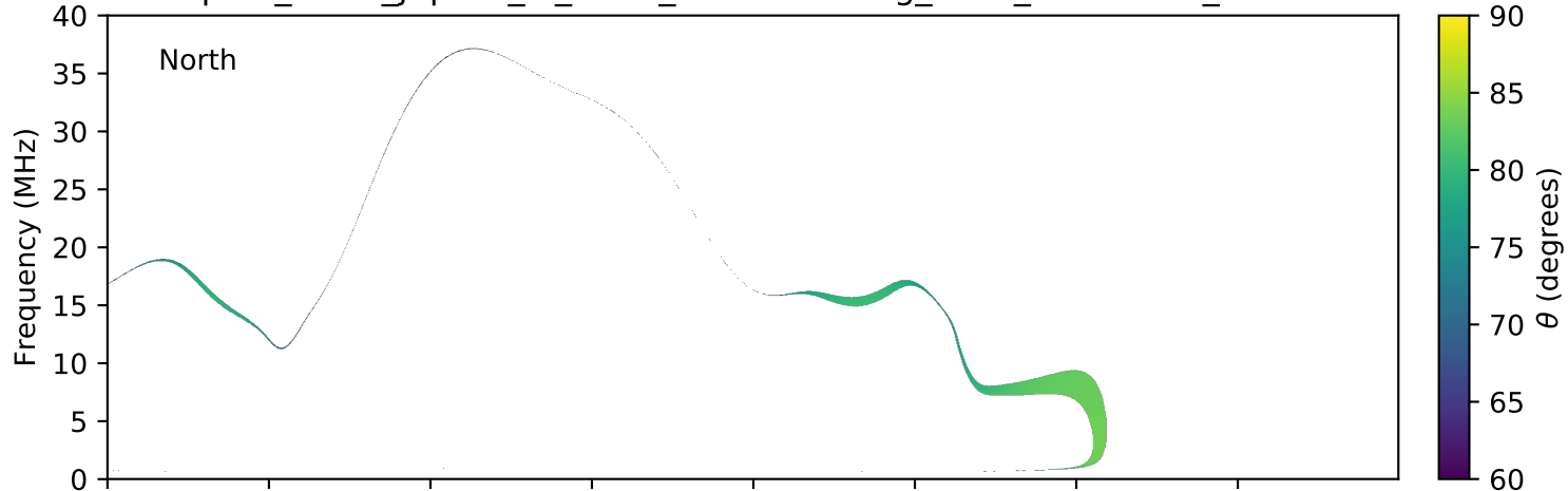
expres_earth_jupiter_io_isaac_lossc-wid1deg_3kev_20050717_v01.cdf
