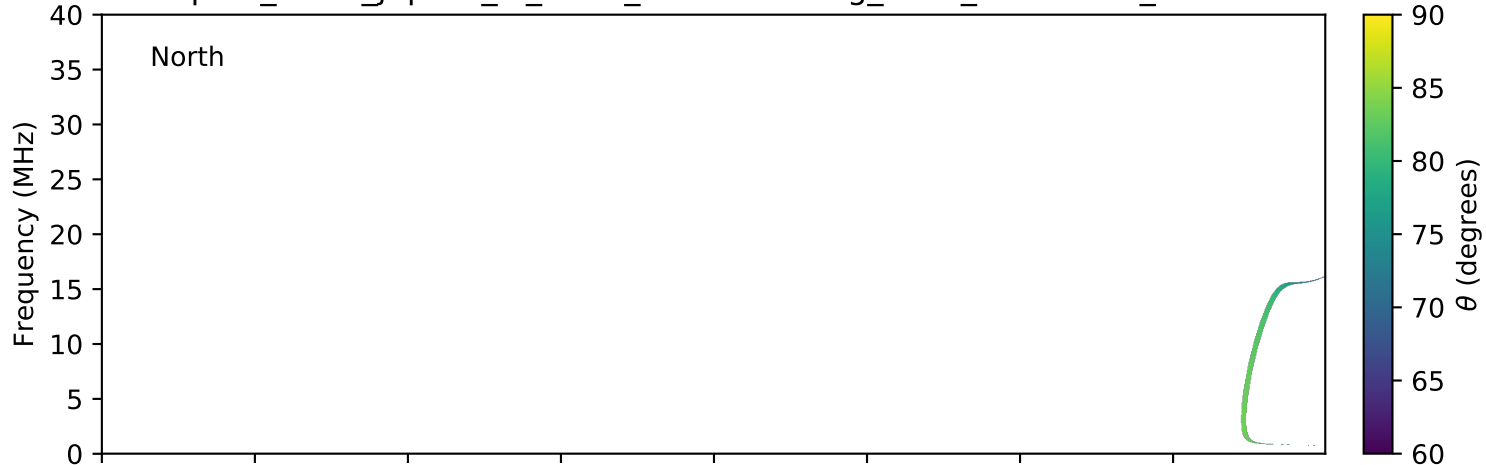
expres_earth_jupiter_io_isaac_lossc-wid1deg_3kev_20050716_v01.cdf
