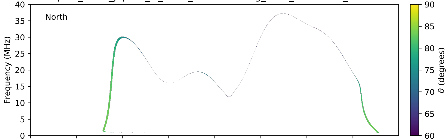
expres_earth_jupiter_io_isaac_lossc-wid1deg_3kev_20050715_v01.cdf
