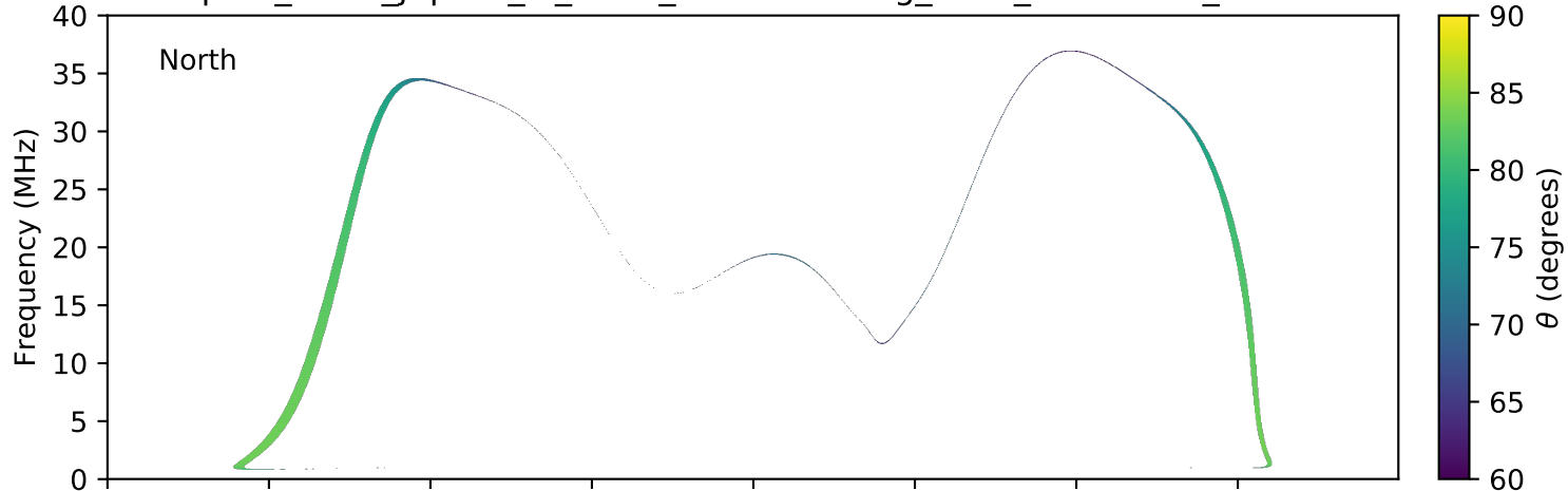
expres_earth_jupiter_io_isaac_lossc-wid1deg_3kev_20050708_v01.cdf
