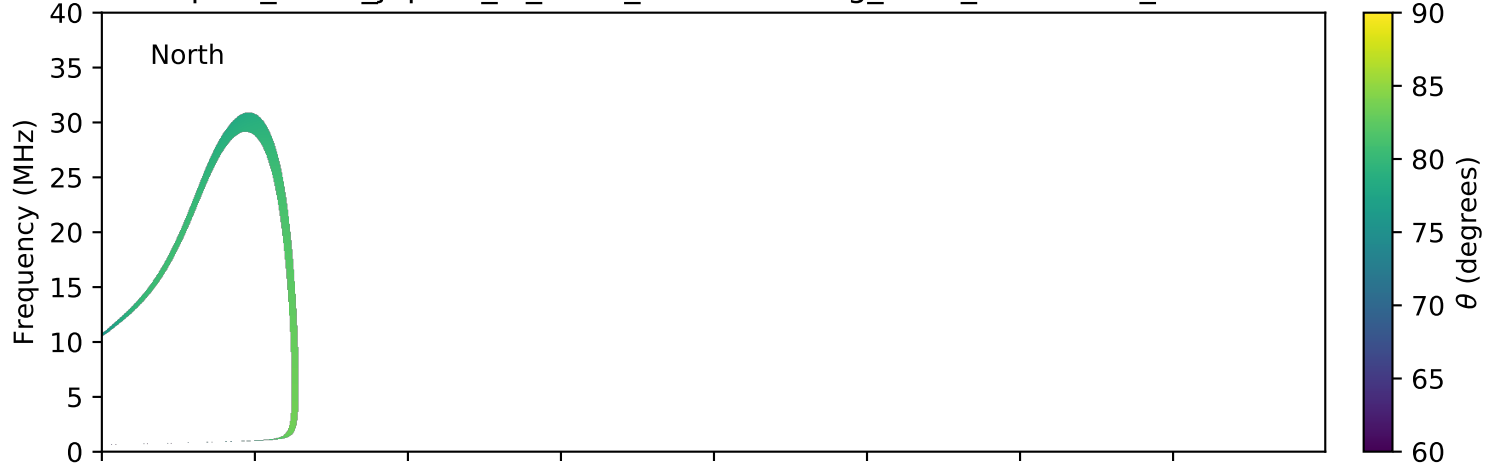
expres_earth_jupiter_io_isaac_lossc-wid1deg_3kev_20050707_v01.cdf
