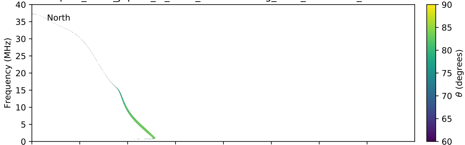
expres_earth_jupiter_io_isaac_lossc-wid1deg_3kev_20050705_v01.cdf
