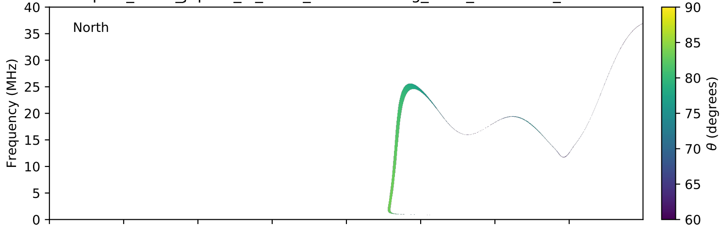
expres_earth_jupiter_io_isaac_lossc-wid1deg_3kev_20050704_v01.cdf
