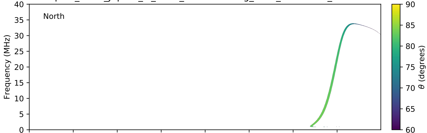
expres_earth_jupiter_io_isaac_lossc-wid1deg_3kev_20050702_v01.cdf
