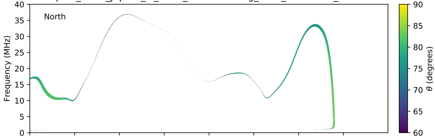
expres_earth_jupiter_io_isaac_lossc-wid1deg_3kev_20050701_v01.cdf
