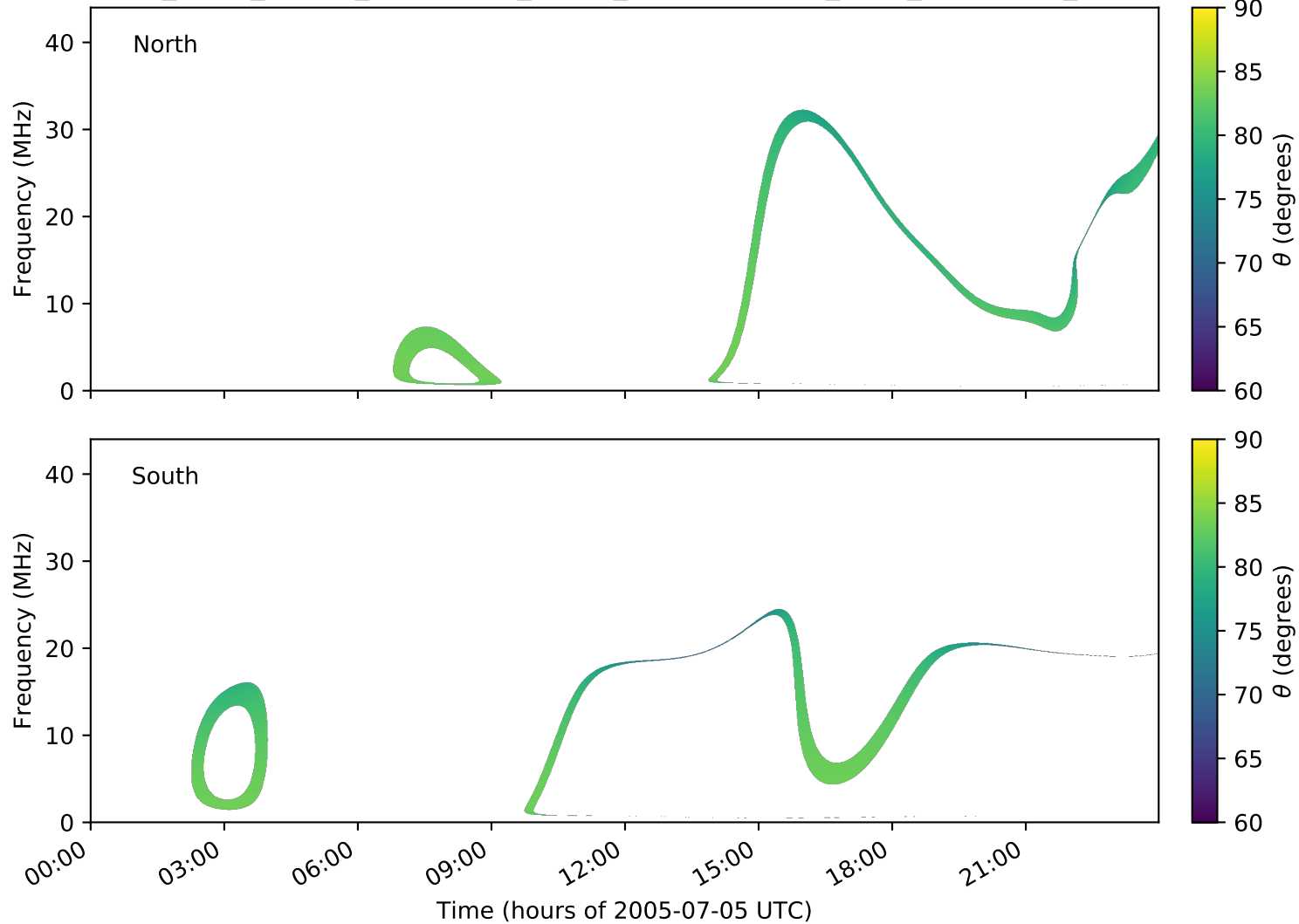
expres_earth_jupiter_ganymede_jrm09_lossc-wid1deg_3kev_20050705_v01.cdf
