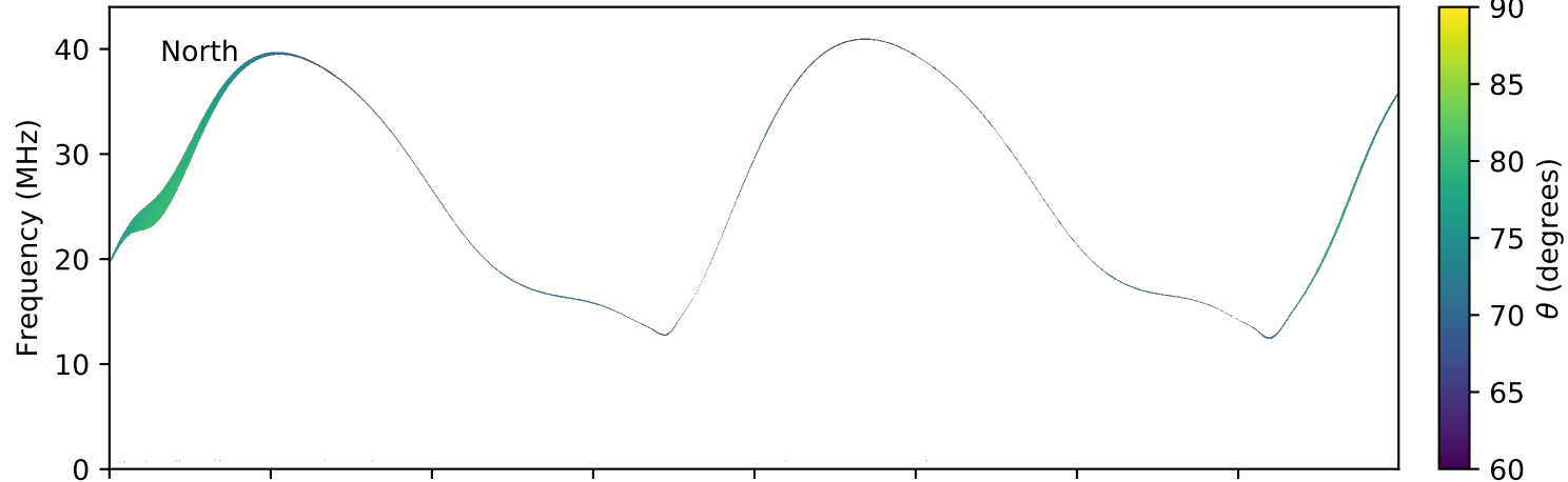
expres_earth_jupiter_europa_jrm09_lossc-wid1deg_3kev_20050708_v01.cdf
