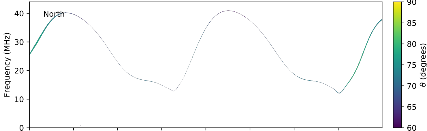
expres_earth_jupiter_europa_jrm09_lossc-wid1deg_3kev_20050701_v01.cdf
