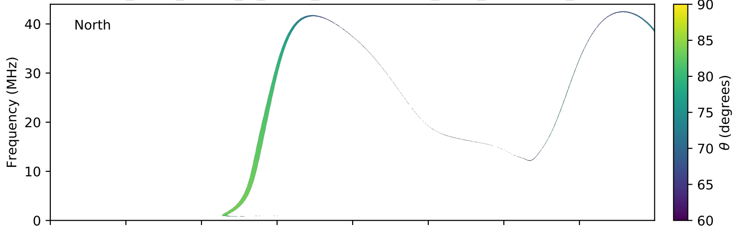
expres_earth_jupiter_io_jrm09_lossc-wid1deg_3kev_20050629_v01.cdf
