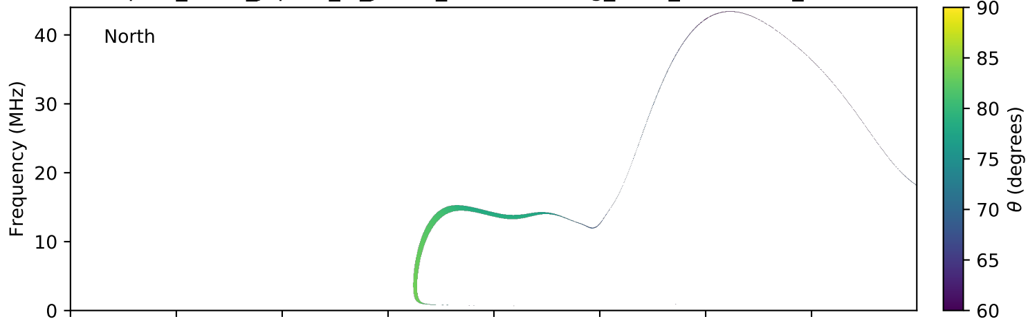
expres_earth_jupiter_io_jrm09_lossc-wid1deg_3kev_20050620_v01.cdf
