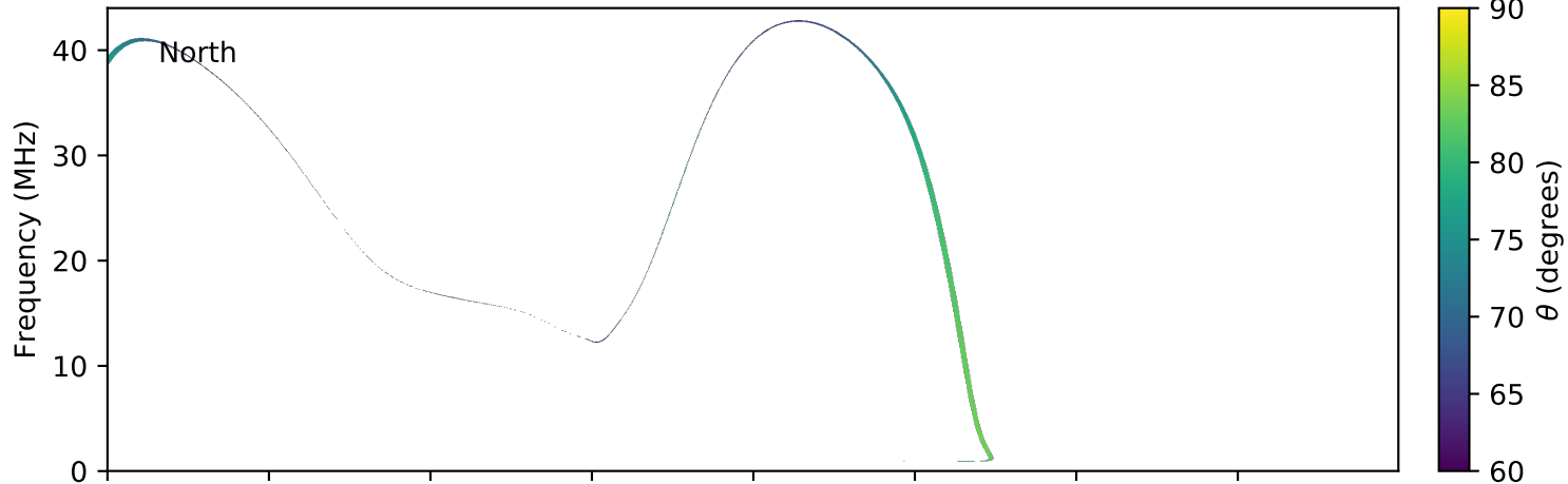
expres_earth_jupiter_io_jrm09_lossc-wid1deg_3kev_20050617_v01.cdf
