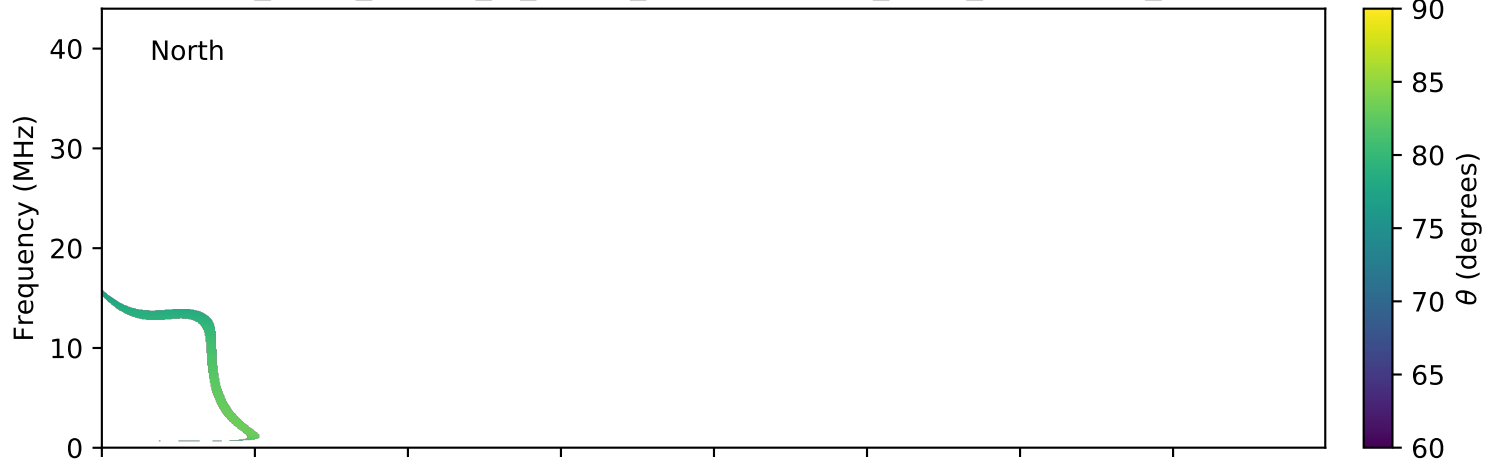
expres_earth_jupiter_io_jrm09_lossc-wid1deg_3kev_20050614_v01.cdf
