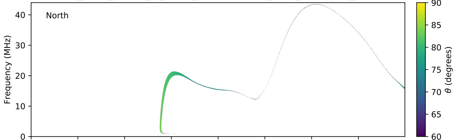
expres_earth_jupiter_io_jrm09_lossc-wid1deg_3kev_20050613_v01.cdf
