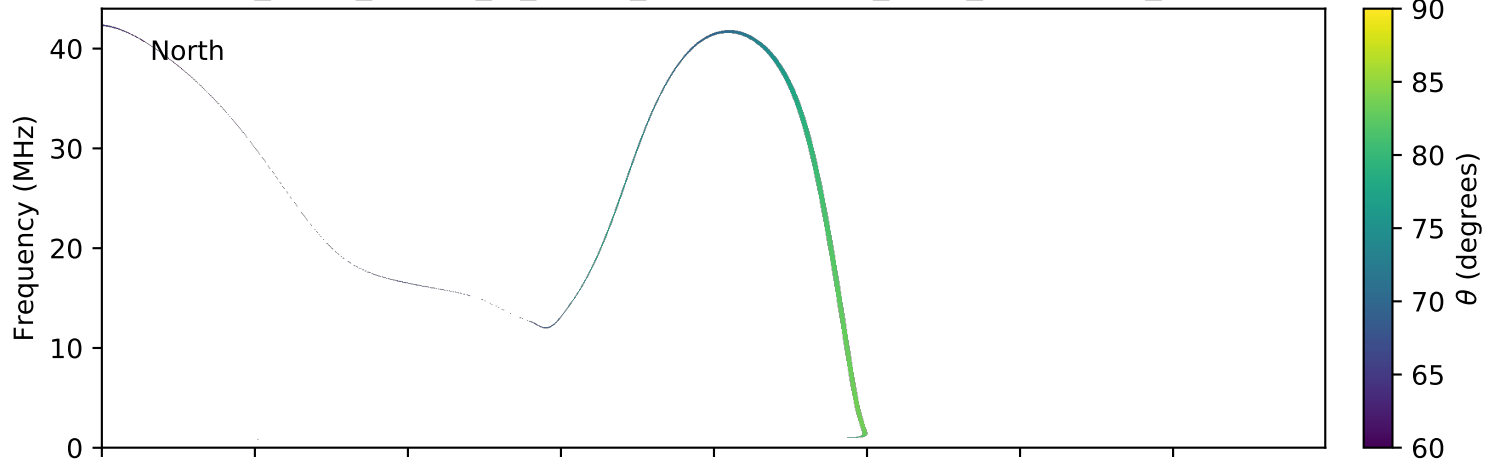
expres_earth_jupiter_io_jrm09_lossc-wid1deg_3kev_20050610_v01.cdf
