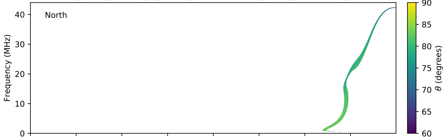
expres_earth_jupiter_io_jrm09_lossc-wid1deg_3kev_20050609_v01.cdf
