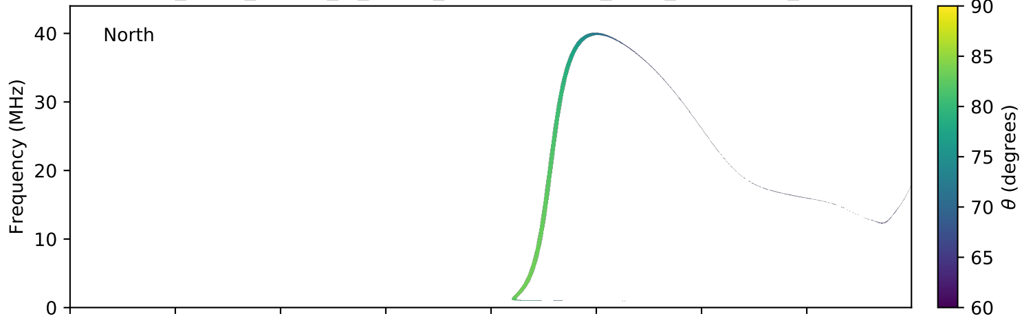
expres_earth_jupiter_io_jrm09_lossc-wid1deg_3kev_20050604_v01.cdf
