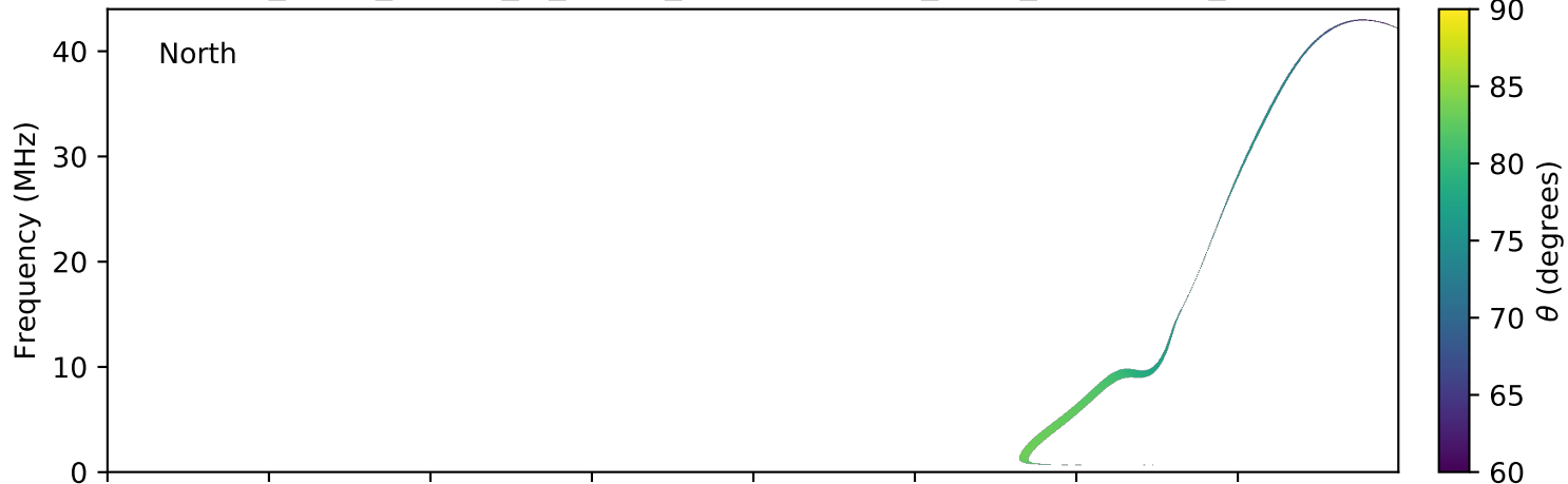
expres_earth_jupiter_io_jrm09_lossc-wid1deg_3kev_20050602_v01.cdf
