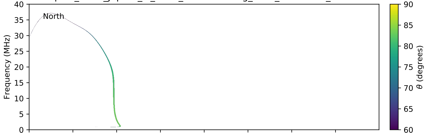
expres_earth_jupiter_io_isaac_lossc-wid1deg_3kev_20050628_v01.cdf
