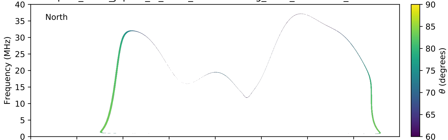
expres_earth_jupiter_io_isaac_lossc-wid1deg_3kev_20050622_v01.cdf
