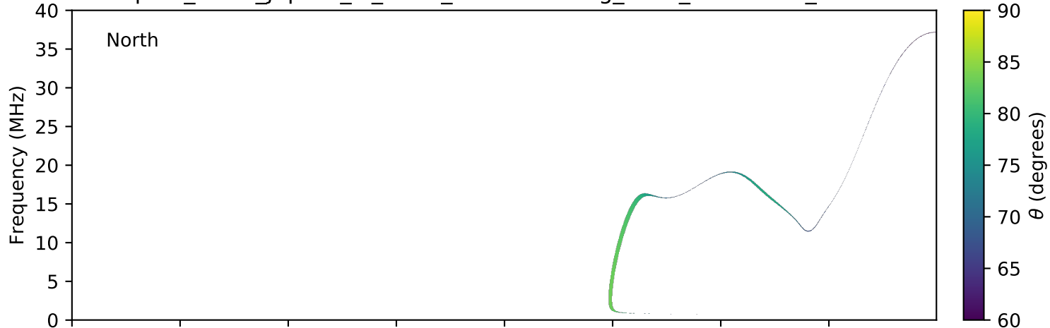
expres_earth_jupiter_io_isaac_lossc-wid1deg_3kev_20050618_v01.cdf
