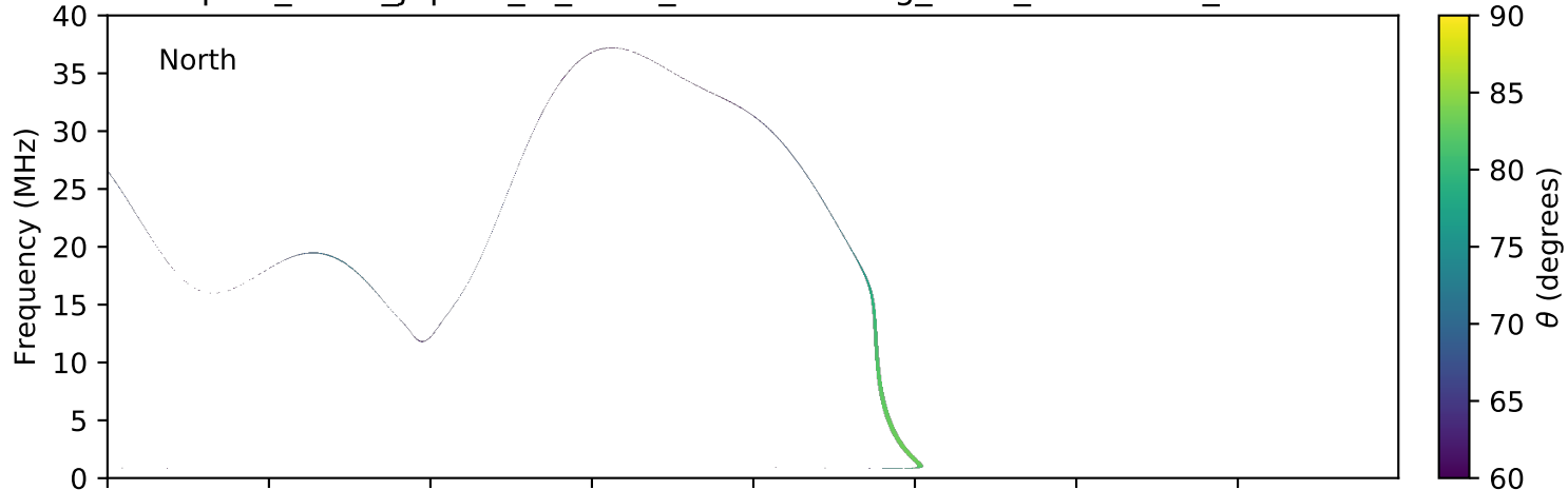
expres_earth_jupiter_io_isaac_lossc-wid1deg_3kev_20050617_v01.cdf
