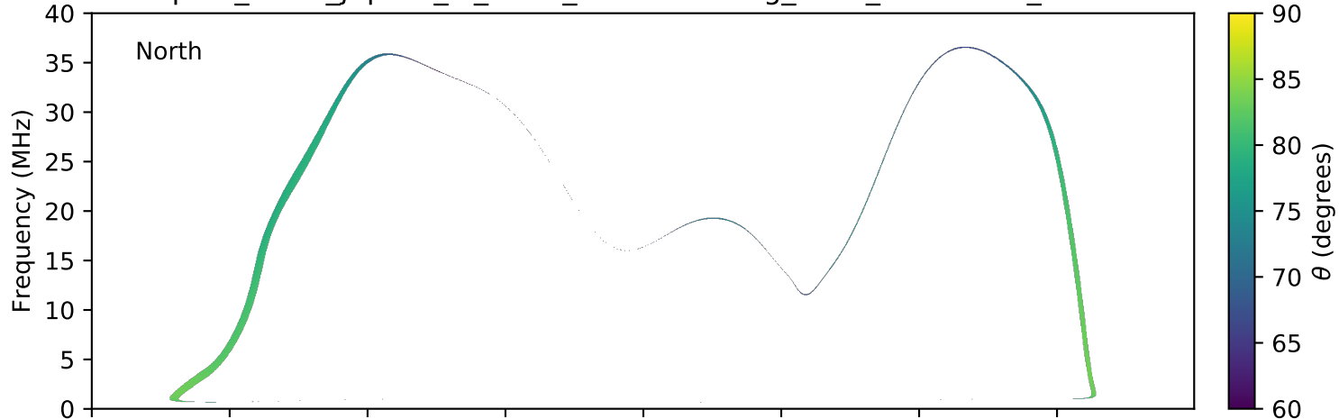
expres_earth_jupiter_io_isaac_lossc-wid1deg_3kev_20050615_v01.cdf
