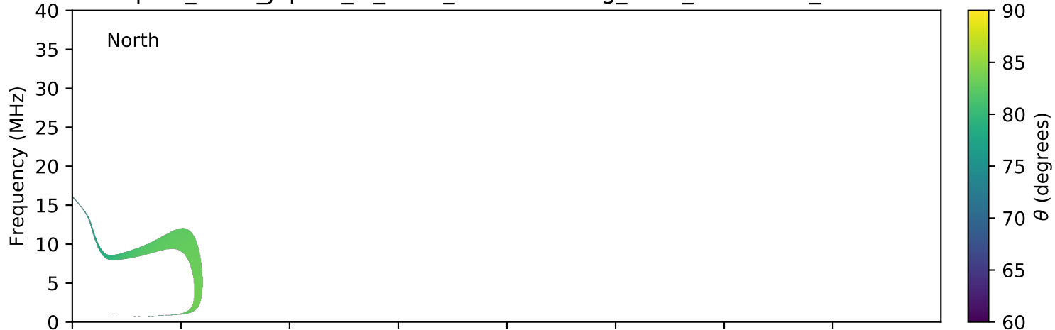
expres_earth_jupiter_io_isaac_lossc-wid1deg_3kev_20050614_v01.cdf
