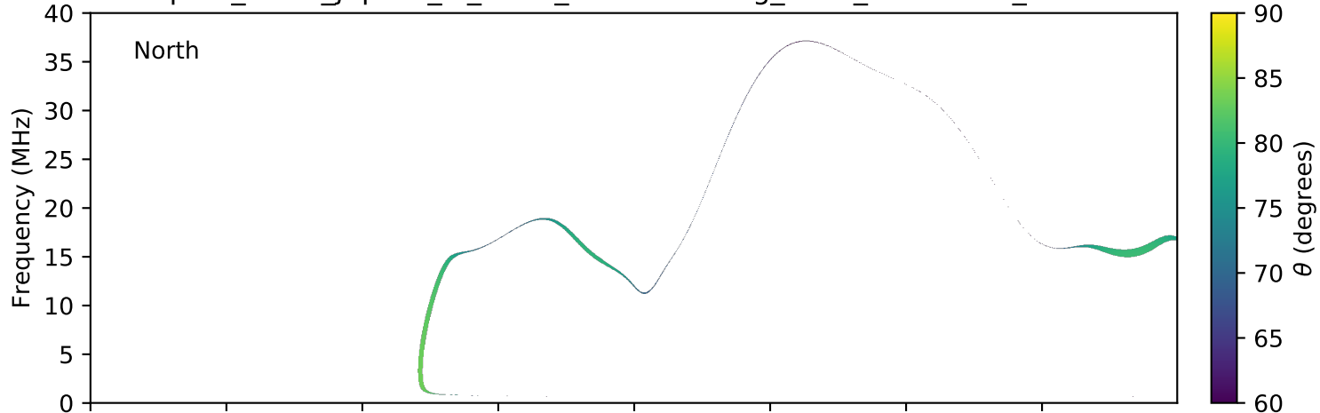
expres_earth_jupiter_io_isaac_lossc-wid1deg_3kev_20050613_v01.cdf
