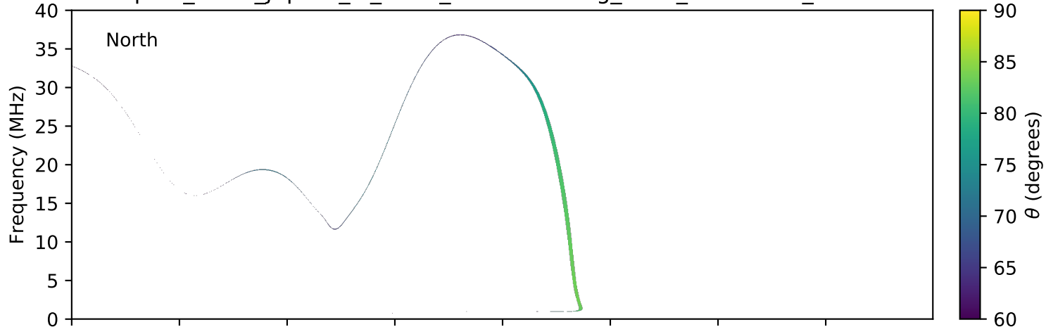
expres_earth_jupiter_io_isaac_lossc-wid1deg_3kev_20050610_v01.cdf
