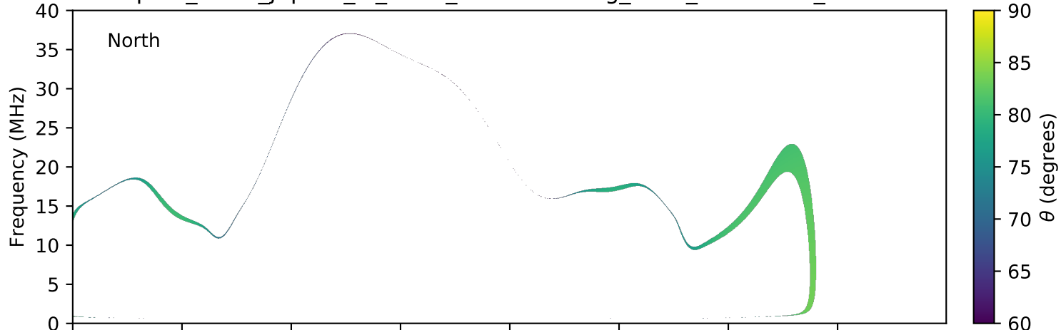
expres_earth_jupiter_io_isaac_lossc-wid1deg_3kev_20050608_v01.cdf
