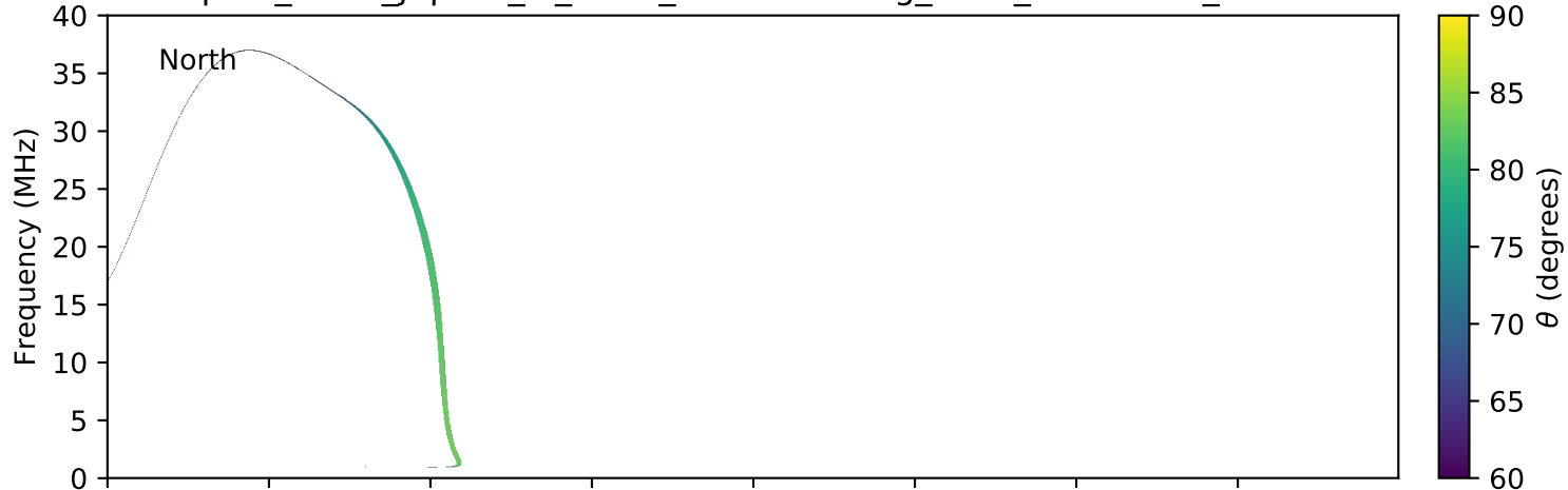
expres_earth_jupiter_io_isaac_lossc-wid1deg_3kev_20050605_v01.cdf
