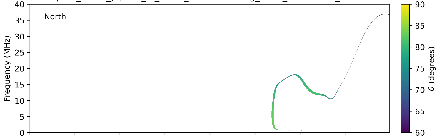
expres_earth_jupiter_io_isaac_lossc-wid1deg_3kev_20050602_v01.cdf
