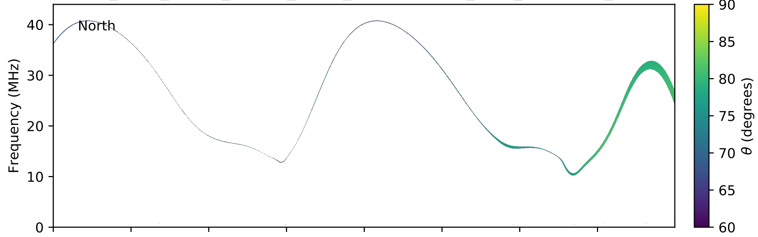
expres_earth_jupiter_europa_jrm09_lossc-wid1deg_3kev_20050617_v01.cdf
