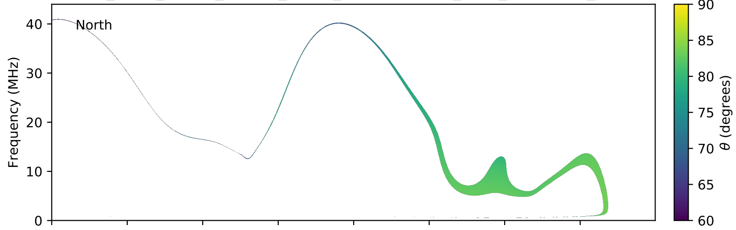
expres_earth_jupiter_europa_jrm09_lossc-wid1deg_3kev_20050603_v01.cdf
