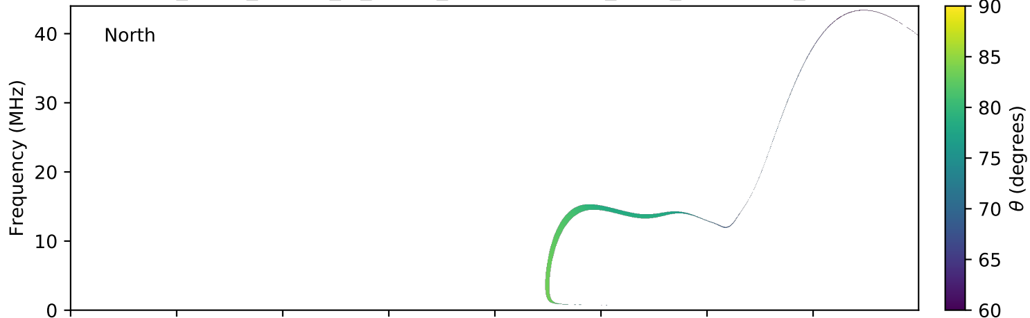
expres_earth_jupiter_io_jrm09_lossc-wid1deg_3kev_20050519_v01.cdf
