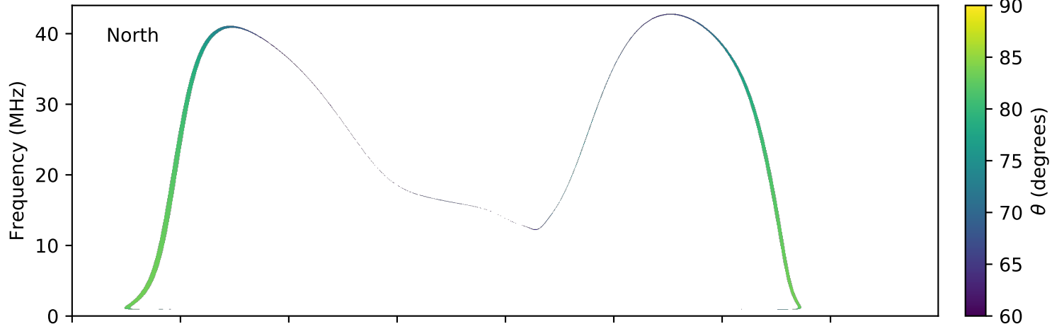
expres_earth_jupiter_io_jrm09_lossc-wid1deg_3kev_20050516_v01.cdf
