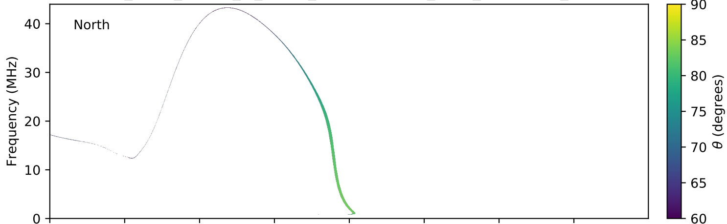
expres_earth_jupiter_io_jrm09_lossc-wid1deg_3kev_20050511_v01.cdf
