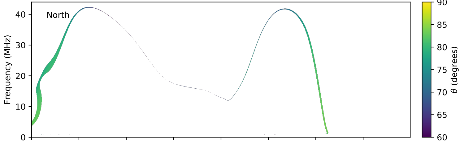
expres_earth_jupiter_io_jrm09_lossc-wid1deg_3kev_20050509_v01.cdf
